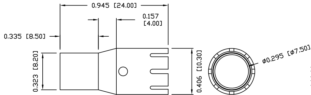
BACK SHELL
