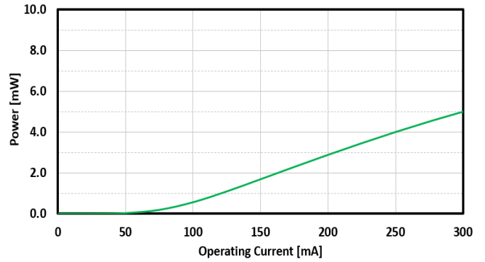
FIG. 8: SLED 1 OUTPUT POWER VS CURRENT
