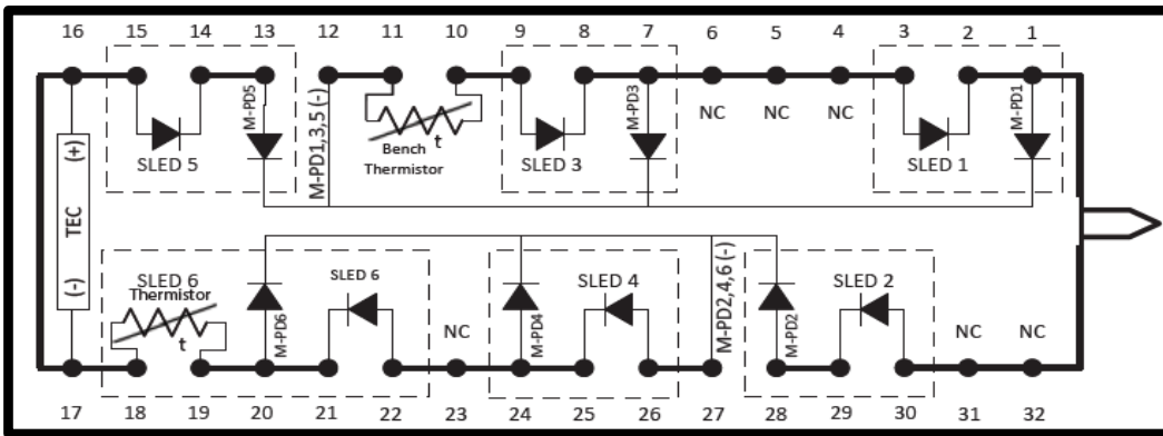
External Pin Assignment – BeST-SLED: 6 SLEDs
