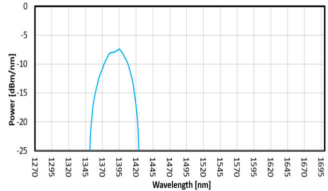
FIG. 6: SLED 5 SPECTRUM
