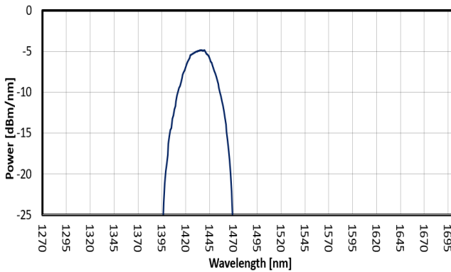
FIG. 5: SLED 4 SPECTRUM
