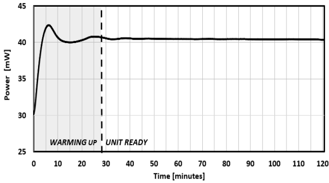
FIG. 15: WARM-UP TIME
