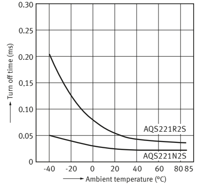
5. Turn off time vs. ambient temperature characteristics
