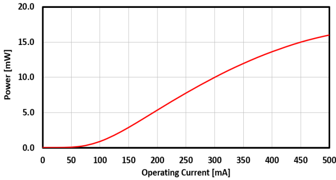
FIG. 9: SLED 3 OUTPUT POWER VS CURRENT
