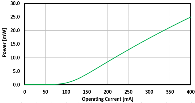
FIG. 7: SLED 1 OUTPUT POWER VS CURRENT
