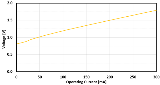
FIG. 13: SLED 2 FORWARD VOLTAGE VS CURRENT
