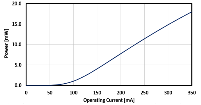
FIG. 10: SLED 4 OUTPUT POWER VS CURRENT
