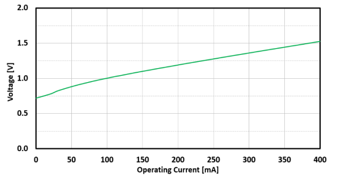
FIG. 12: SLED 1 FORWARD VOLTAGE VS CURRENT
