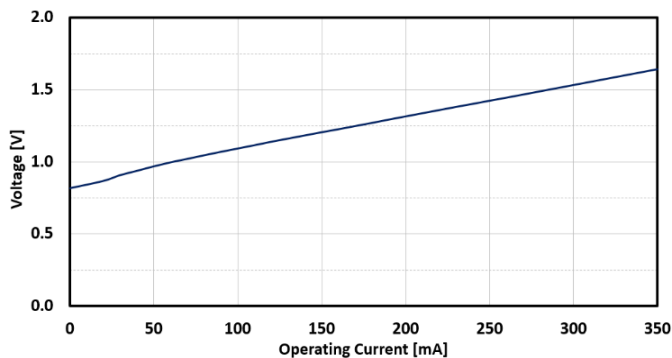
FIG. 15: SLED 4 FORWARD VOLTAGE VS CURRENT
