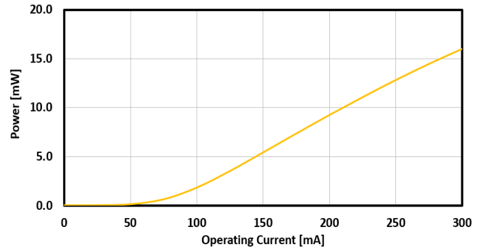
FIG. 8: SLED 2 OUTPUT POWER VS CURRENT
