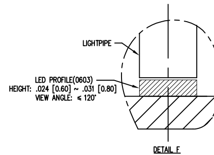
DETAIL F
