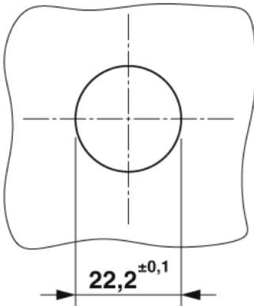
Dimensional drawing
