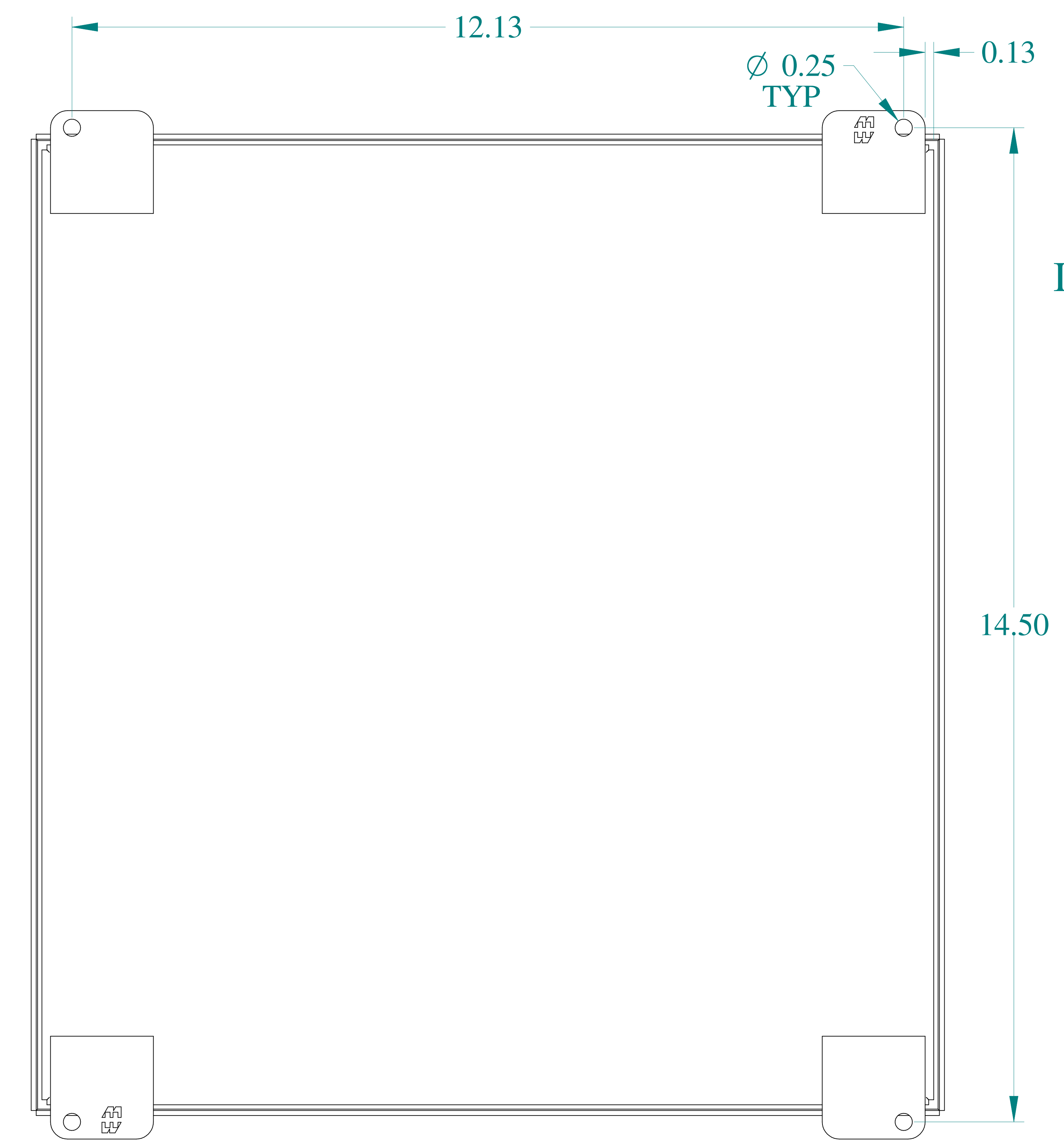
BACK VIEW
