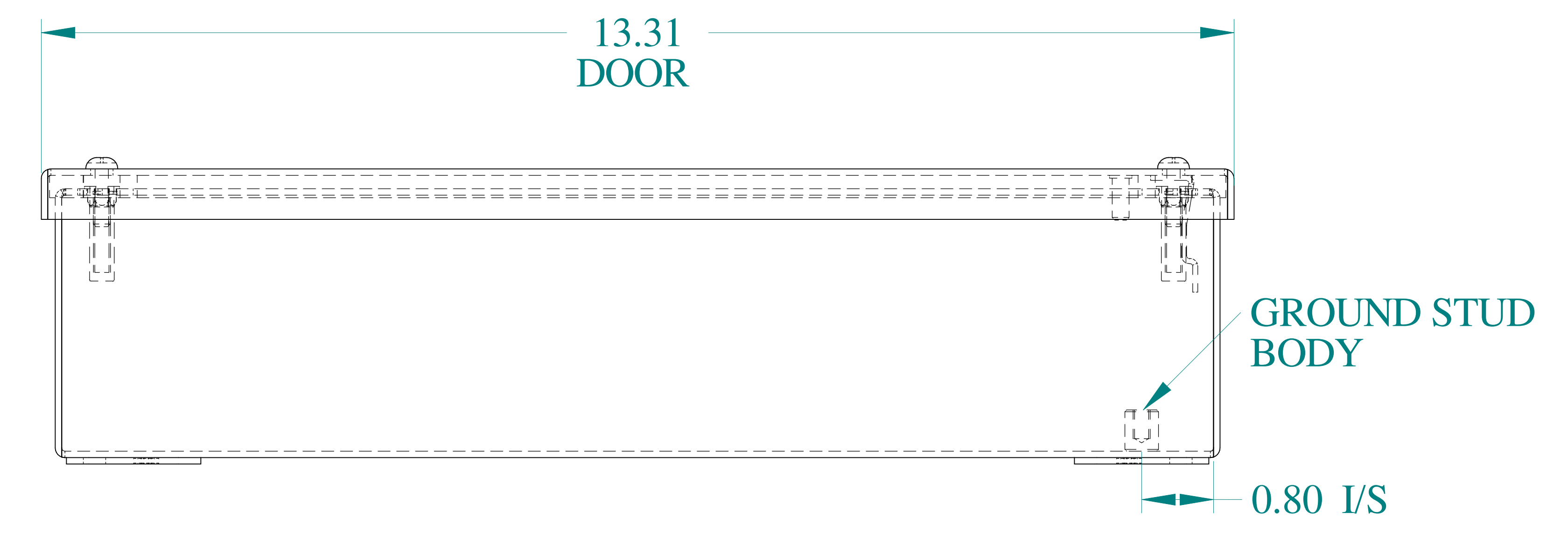
BOTTOM VIEW
