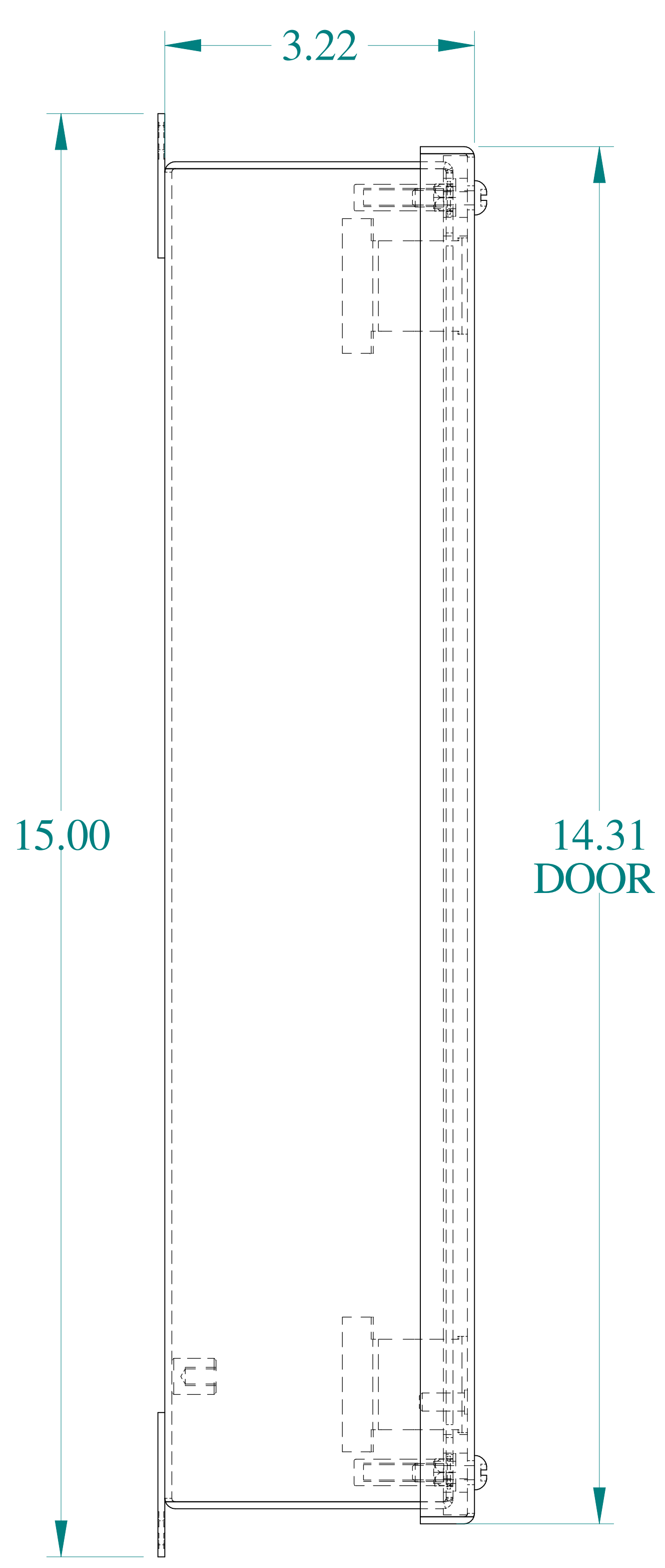
SIDE VIEW
