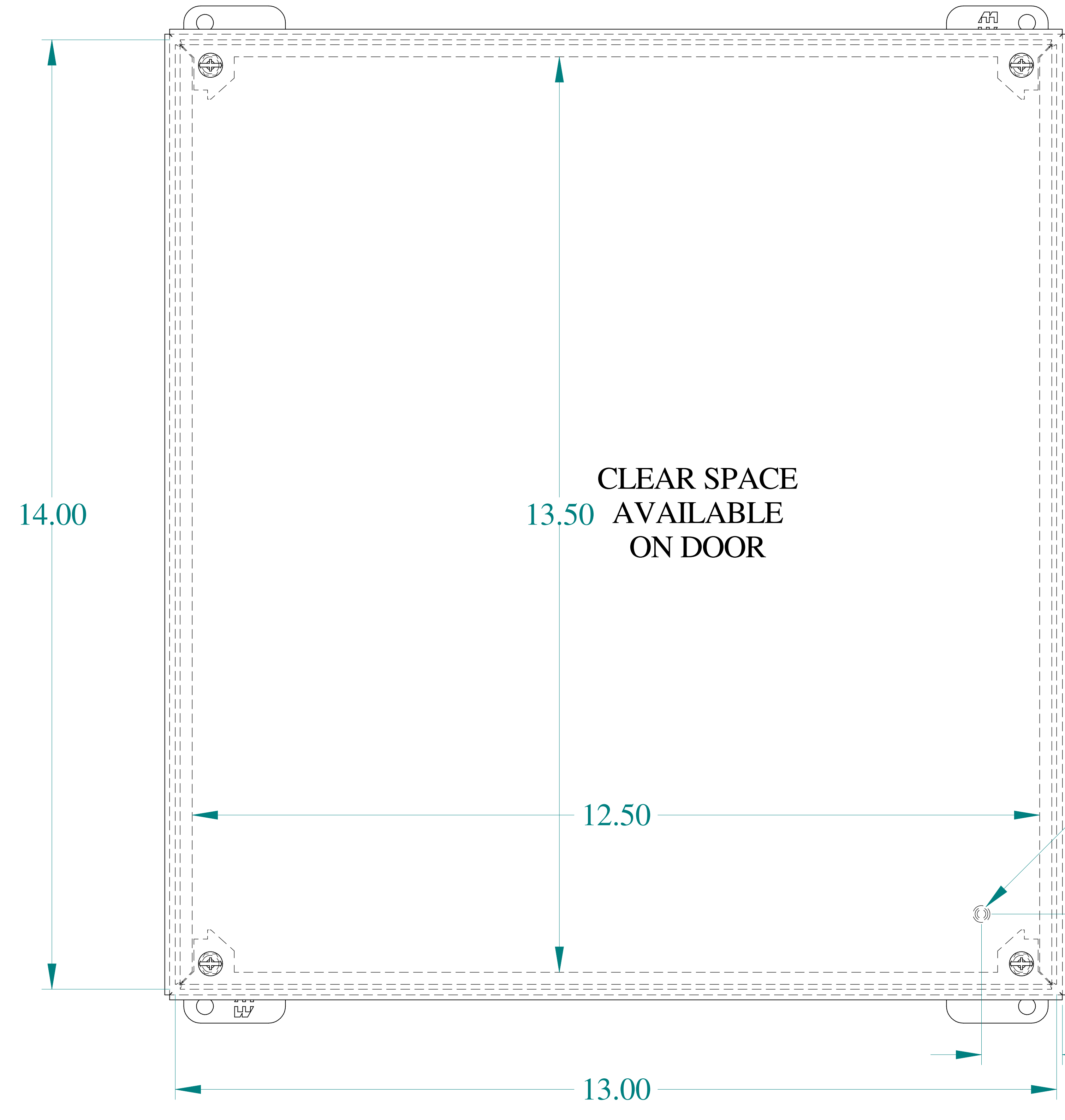
FRONT VIEW
