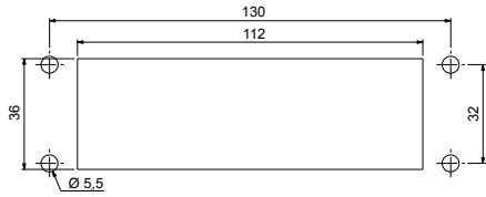
Cut-out for reference NSYDCE24●●●
