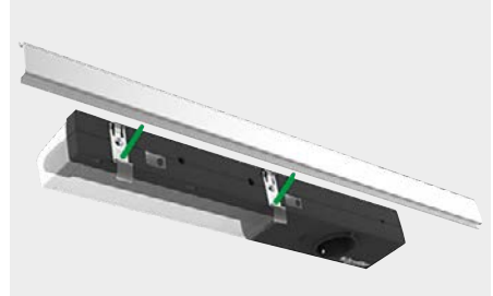
Fixing to DIN rail.
