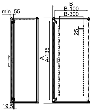
Models with a width of 1200 mm without top/bottom adjustment rails
