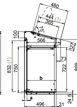
Cable gland plate clearance dimensions (mm)
