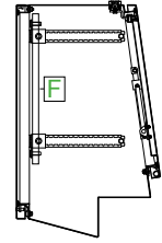
Example installation of a mounting plate in a console depth 300 mm.
