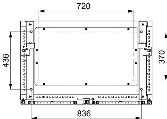
Enclosure width 1000
