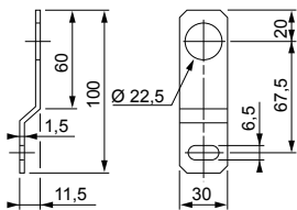
Ø 22 mm cable-duct support
