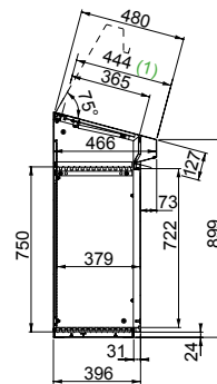
Cable gland plate clearance dimensions (mm)
