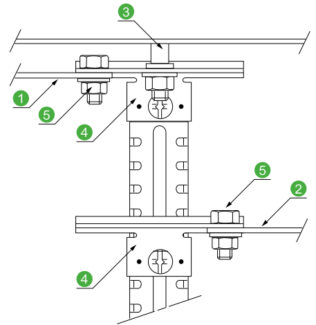
2 Two offset mounting plates with depthwise adjustment
