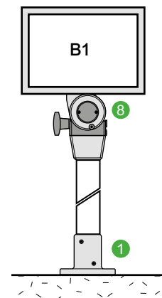
Fixing on support 1 See page 511 Inter-tube fitting Fixing on enclosure 8 See page 512
