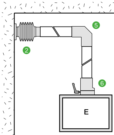
Fixing on support 2 See page 511 Inter-tube fitting 5 See page 512 Fixing on enclosure 6 See page 512
