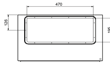
Cable entry type G: Enclosure width 600 mm.
