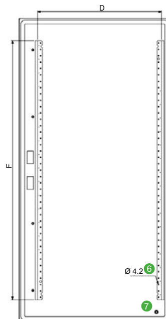
Cable entry type G: Enclosure width 600 mm.
