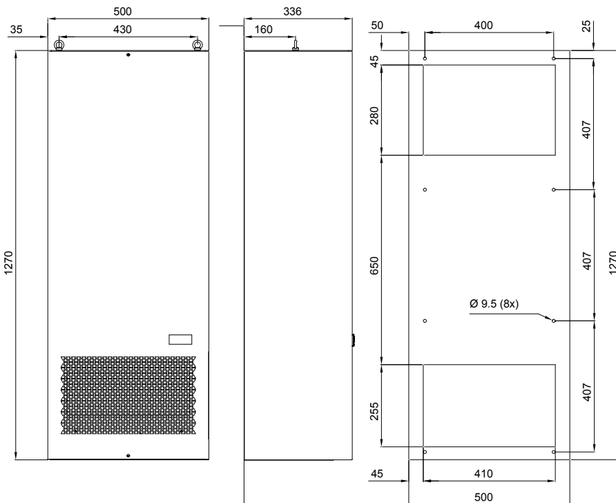
NSYCU●●3K3P4●● - NSYCU●●4K3P4●●
