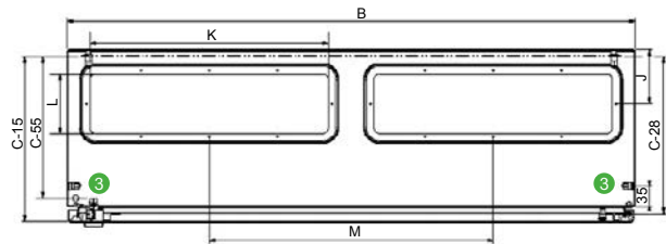
Cable entry type H: Enclosure width \geq 800 mm.
