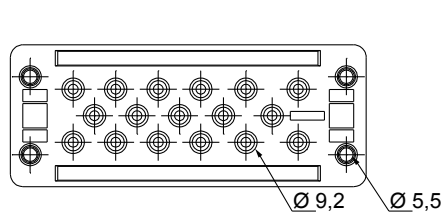
NSYTSA2417SE
