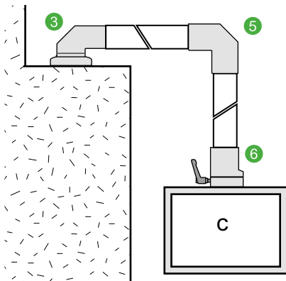
Fixing on support 3 See page 511 Inter-tube fitting 5 See page 512 Fixing on enclosure 6 See page 512
