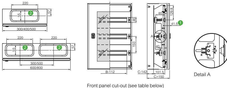
Front panel cut-out (see table below)
