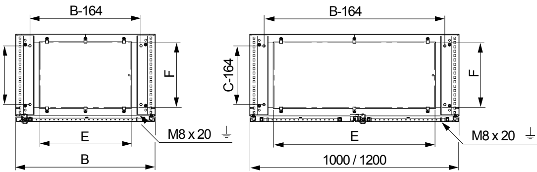
Enclosure width of 1000 and 1200 mm
