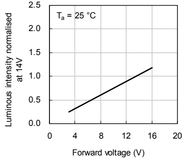
Luminous Intensity vs. Forward Voltage
