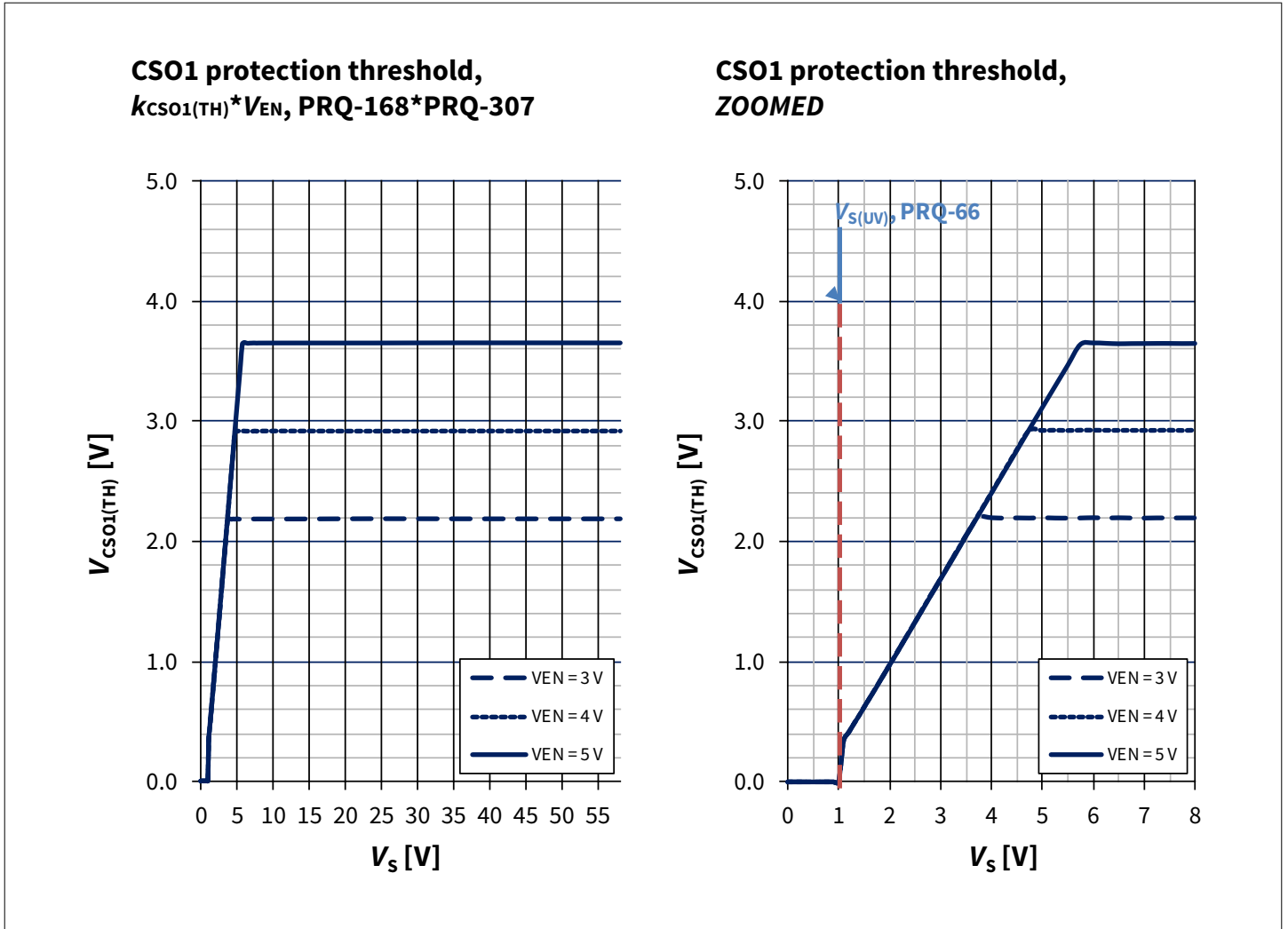
Figure 20 Typical V_{CS01(TH)} versus V_S and V_{EN} (independent of T_J )
