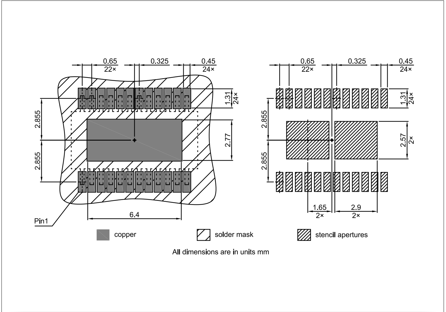
Figure 36 Footprint drawing
