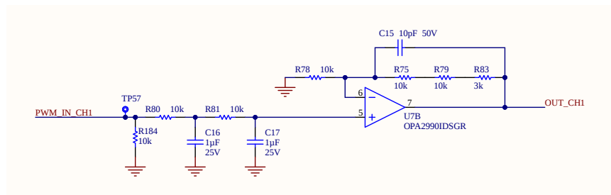
Analog Output Circuit
