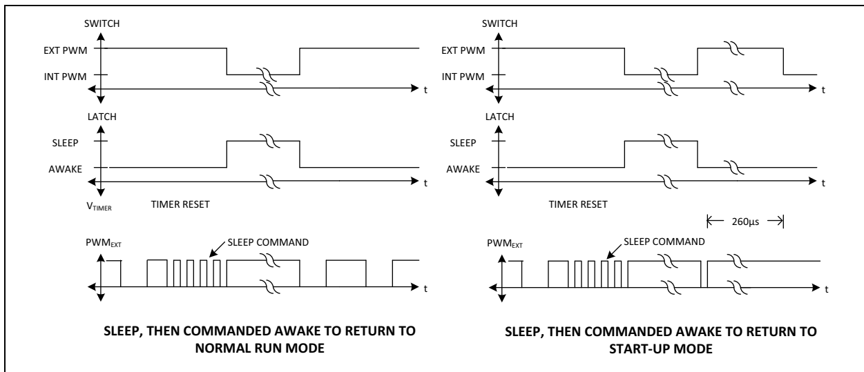
FIGURE 4-8: Externally Comanded to Enter and Exit Sleep Mode.
