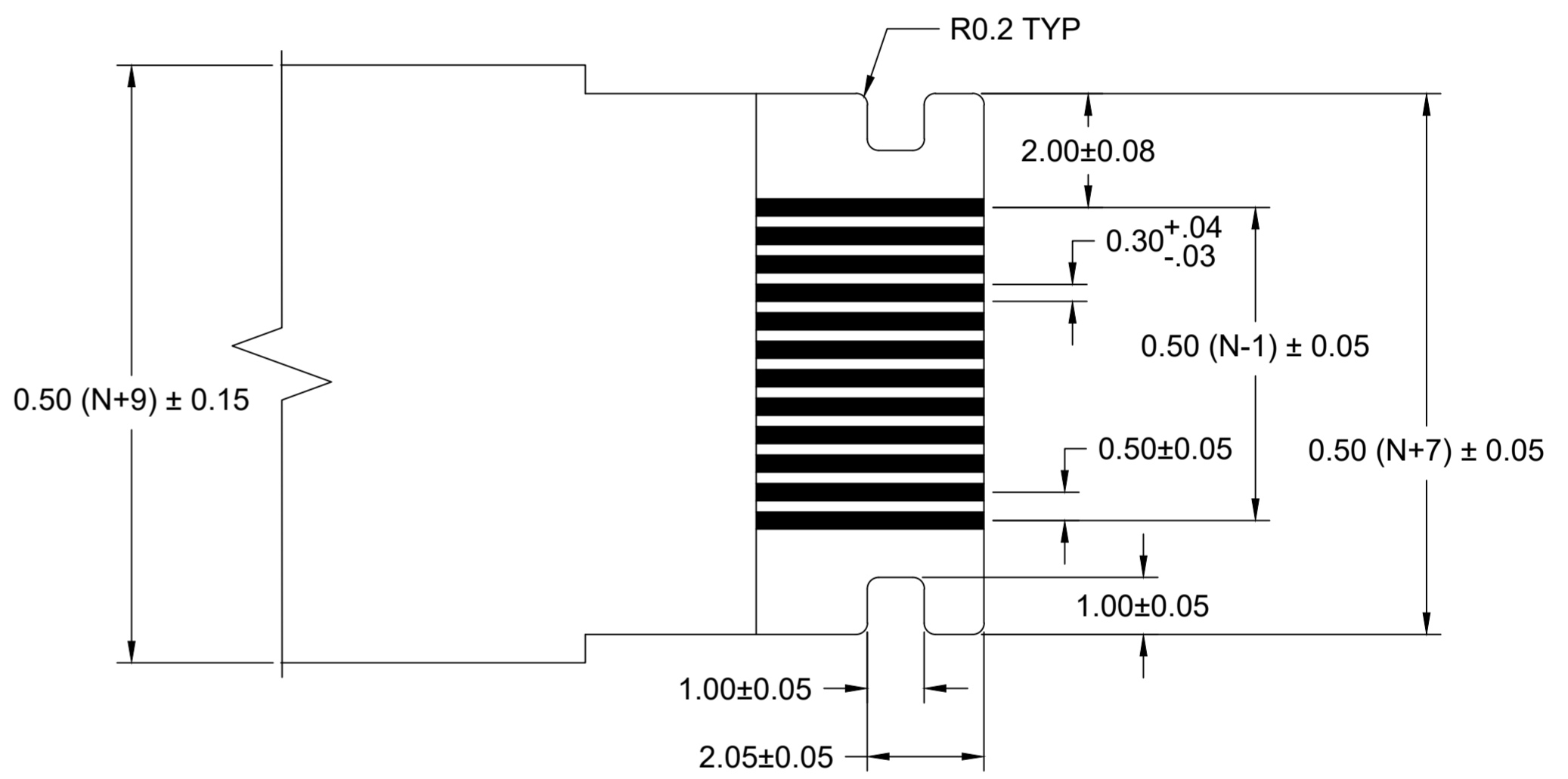
END-TAIL DIMENSIONS SCALE 10:1
