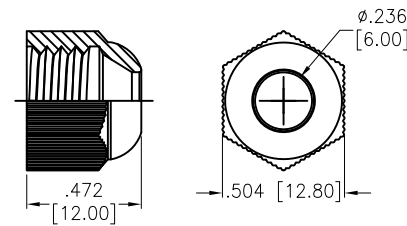
Ⓔ Sealing Nut
