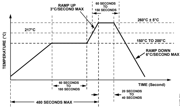
Figure 88. Soldering Profile
