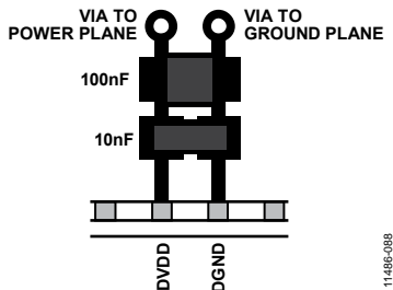
Figure 81. Layout for Multiple Power Supply Bypass Capacitors
