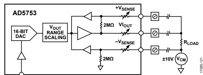
Figure 79. Voltage Output
