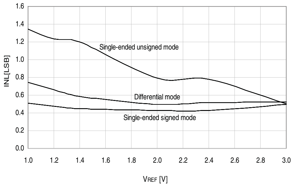
Figure 36-30. INL Error vs. External V_{REF} T = 25^\circ\text{C} , V_{CC} = 3.6\text{V} , external reference
