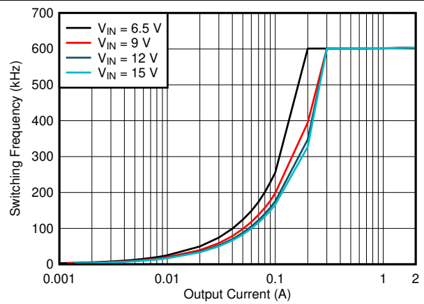
Figure 6-12. Switching Frequency vs Output Current, V OUT = 3.3 V, L = 4.7 μH
