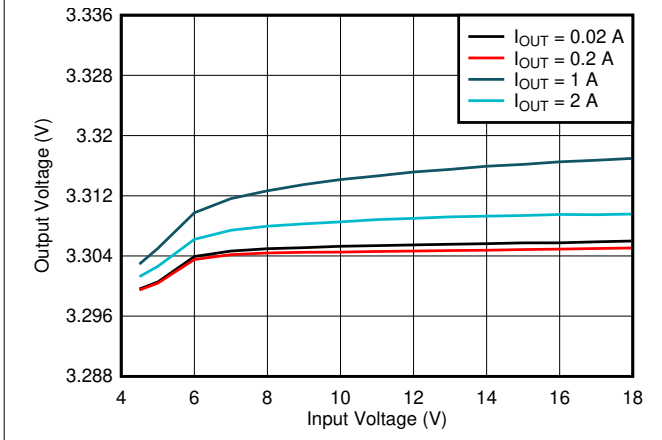
Figure 8-4. Line Regulation
