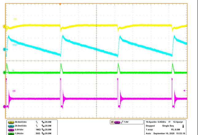
Figure 8-7. Steady State Waveforms, I_{OUT} = 0.02\text{ A}
