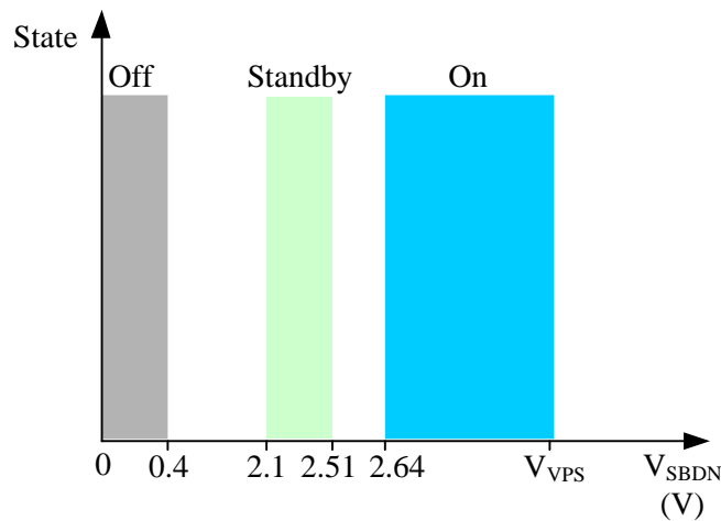
Figure 3. The States of Amplifier vs. V_{\text{SBDN}}
