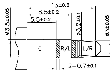
MATE PLUG
