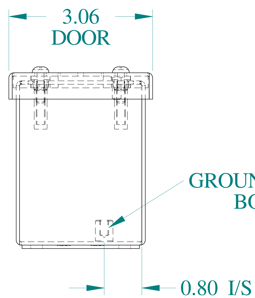
BOTTOM VIEW
