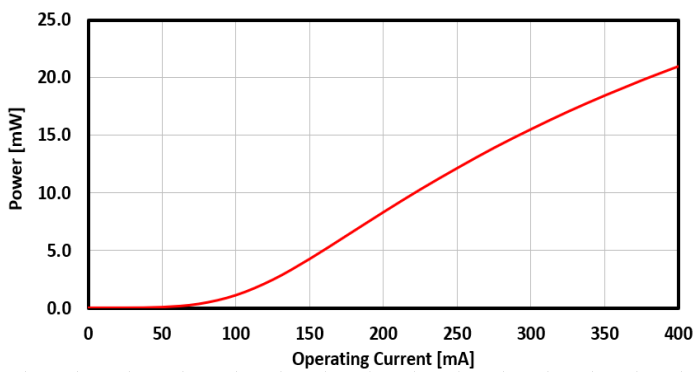
FIG. 7: SLED 3 OUTPUT POWER VS CURRENT
