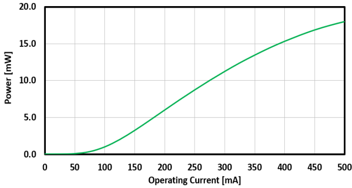
FIG. 5: SLED 1 OUTPUT POWER VS CURRENT
