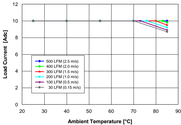
Fig. 5.0V.1: Available load current vs. ambient temperature and airflow rates for V_{out} = 5.0\text{V} converter mounted vertically with V_{in} = 12\text{V} , and maximum MOSFET temperature \leq 120^{\circ}\text{C} .
