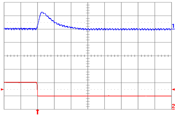
Fig. 2.5V.8: Output voltage response for V_{out} = 2.5V to negative load current step change from 10A to 5A with slew rate of -5A/\mu s at V_{in} = 12V . Top trace: output voltage (100mV/div.); Bottom trace: load current (5A/div.). C_o = 100\mu F ceramic. Time scale: 20 \mu s /div.
