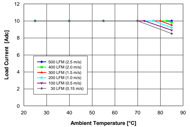
Fig. 5.0V.2: Available load current vs. ambient temperature and airflow rates for V_{out} = 5.0\text{V} converter mounted horizontally with V_{in} = 12\text{V} , and maximum MOSFET temperature \leq 120^{\circ}\text{C} .
