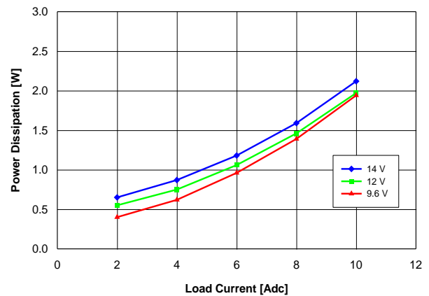
Fig. 1.2V.4: Power Loss vs. load current and input voltage for V_{out} = 1.2V converter mounted vertically with air flowing at a rate of 200 LFM (1 m/s) and T_a = 25^{\circ}C .
