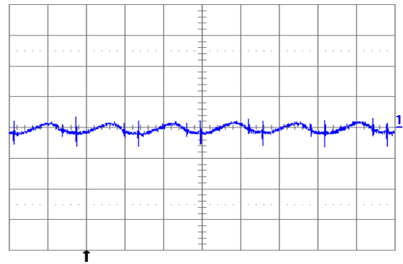
Fig. 2.5V.6: Output voltage ripple (20mV/div.) at full rated load current into a resistive load with external capacitance 100\mu F ceramic and V_{in} = 12V for V_{out} = 2.5V . Time scale: 2 \mu s /div.
