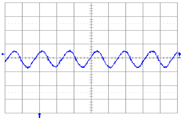
Fig. 5.0V.6: Output voltage ripple (20mV/div.) at full rated load current into a resistive load with external capacitance 100\mu\text{F} ceramic and V_{in} = 12\text{V} for V_{out} = 5.0\text{V} . Time scale: 2µs/div.
