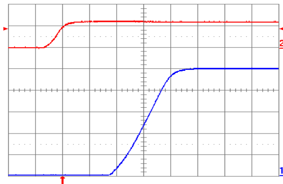
Fig. 5.0V.5: Turn-on transient for V_{out} = 5.0\text{V} with application of V_{in} at full rated load current (resistive) and 100\mu\text{F} external capacitance at V_{in} = 12\text{V} . Top trace: V_{in} (10V/div.); Bottom trace: output voltage (1V/div.); Time scale: 2ms/div.
