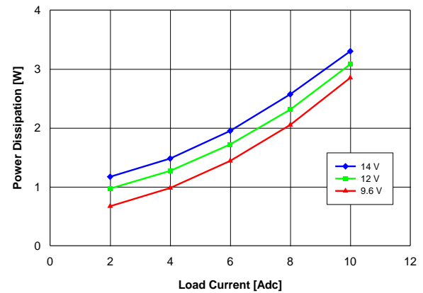
Fig. 5.0V.4: Power Loss vs. load current and input voltage for V_{out} = 5.0\text{V} converter mounted vertically with air flowing at a rate of 200 LFM (1 m/s) and T_a = 25^{\circ}\text{C} .
