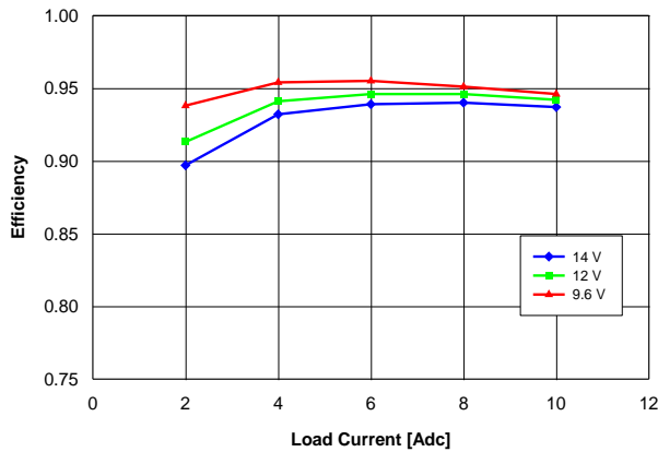
Fig. 5.0V.3: Efficiency vs. load current and input voltage for V_{out} = 5.0\text{V} converter mounted vertically with air flowing at a rate of 200 LFM (1 m/s) and T_a = 25^{\circ}\text{C} .
