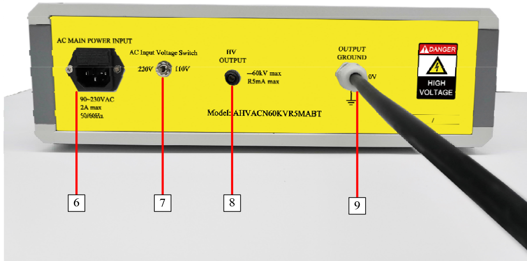
Figure 3. Front Panel
