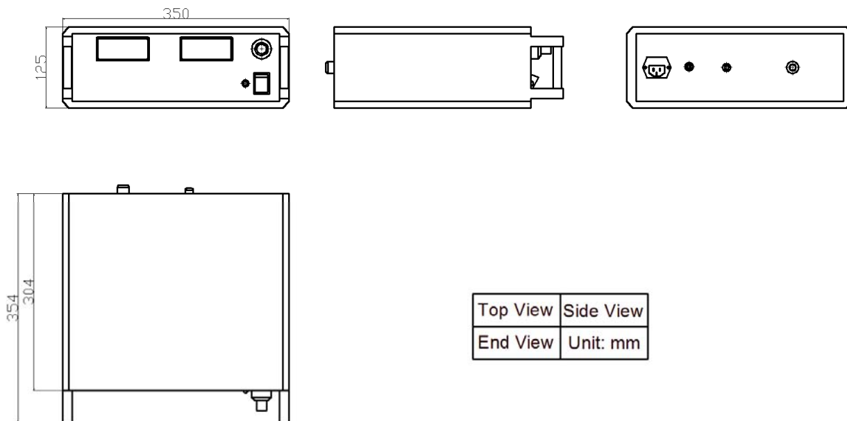
Figure 7. Dimensions for AHVACN60KVR5MABT
