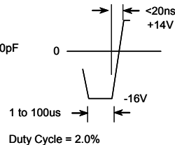
Fig. 2. Turn-Off Time
