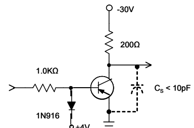
Fig. 2. Turn-Off Time
