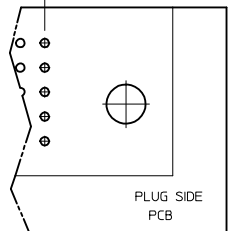
Horizontal Position Partial View SCALE 5:1
