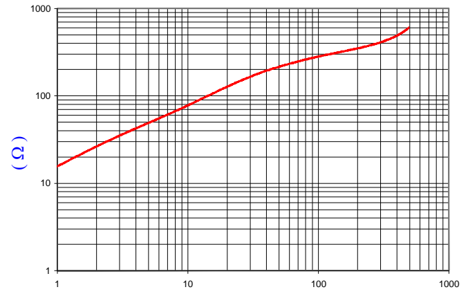
FREQUENCY (MHz) AGILENT E4991A Impedance/Material Analyzer HP 16092A Test Fixture REF #3188
