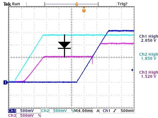
Figure 25 was captured with an actual system where a diode was added to pre-bias a 1.5V bus from a 1.85V bus in order to simulate the effect of current leakage through protection circuits of unpowered logic connected to powered logic outputs (a common source of pre-bias in power systems).
