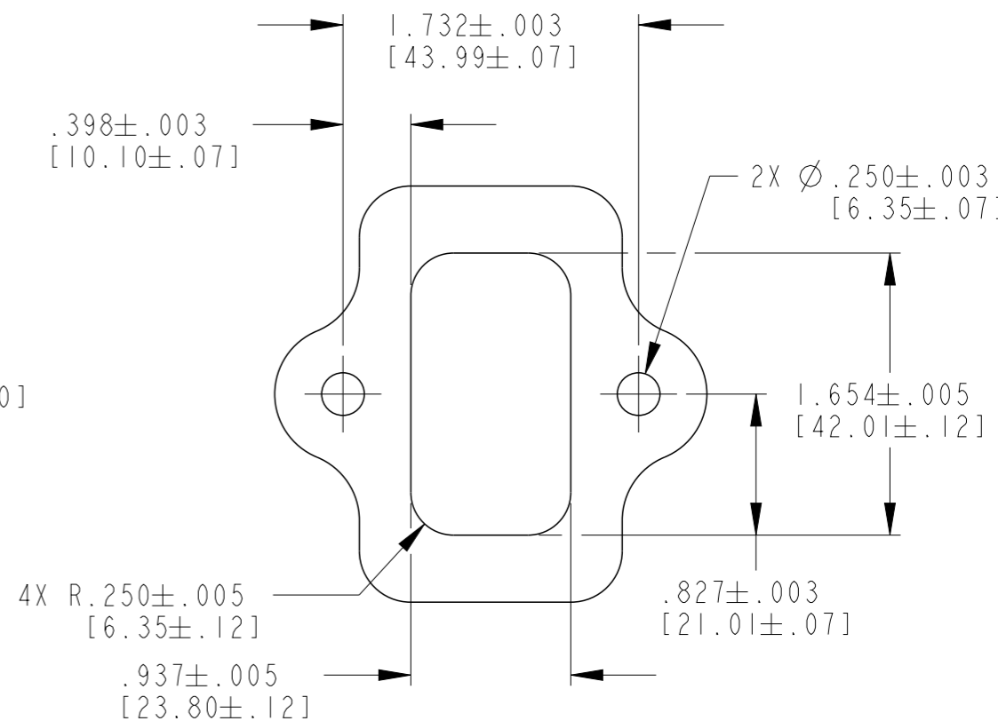
RECOMMENDED MOUNTING DETAIL
