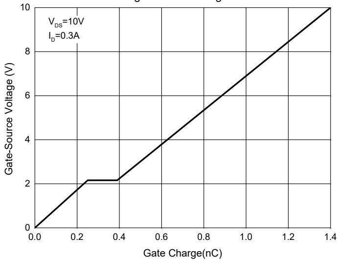
Fig. 7 - Gate Charge
