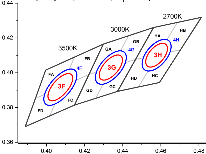
CIE Chromaticity Diagram (Cool white), T_j=85^\circ\text{C} , I_F=100\text{mA}
