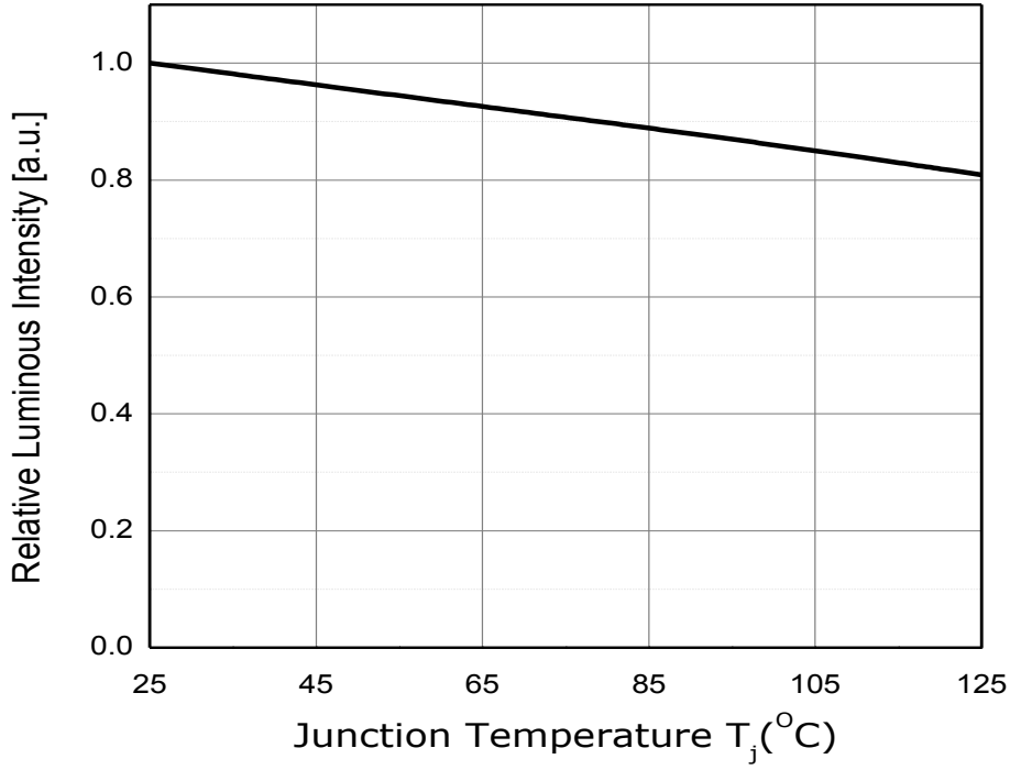
Fig 6. Junction Temperature vs. Relative Luminous Flux, I_F=100\text{mA}
