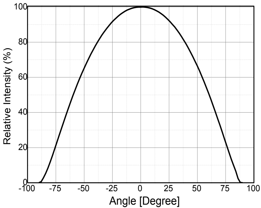
Fig 2. Radiant Pattern, T_j = 25^\circ\text{C} , I_F = 100\text{mA}
