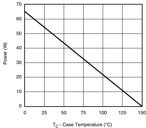
Power, Junction-to-Case
