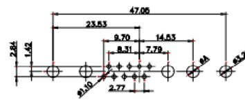
13W3 Female
