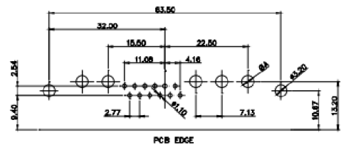
17W5 Male
