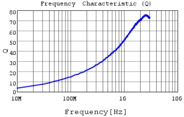
LQG15WH3N4B02 Q
