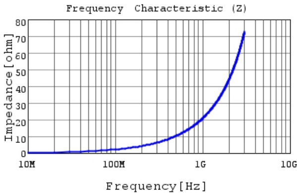
LQG15WH3N4B02 |Z|
