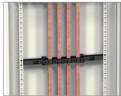
Rear Lineryg BS busbars.
