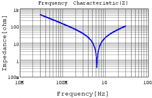
RCE5C2E120J1M1H03A |Z| DC0V, 25degC
