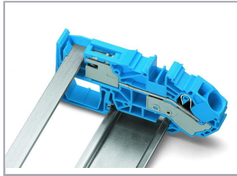
Touch-proof N-busbar via inserted separator plate
