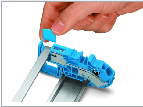
Inserting separator plate removed from N-disconnect terminal block.
