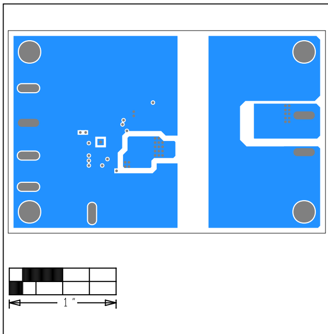
MAX17690 EV Kit—Bottom
