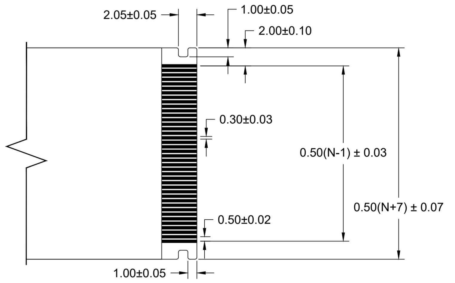
END TAIL DETAIL SCALE 4:1
