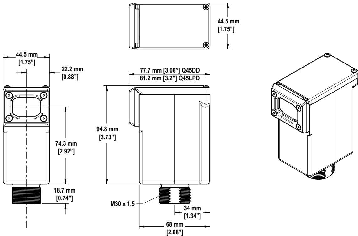
Figure 1: Dimensions for the Q45UPSD
