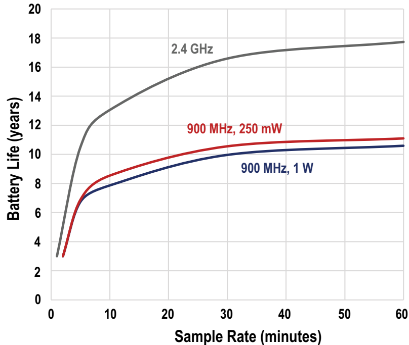
Figure 2: Battery life for the Q45UPSD Node
