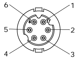
FACE VIEW 16982-6SG-5XX 6 POSITION B-KEY
