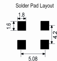
Solder Pad Layout
