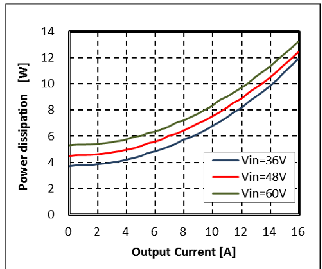
Fig-3: Power dissipation vs. load current and input voltage for converter mounted horizontally with airflow from pin 1 to pin 3 at a rate of 400LFM (2.0m/s) and Ta=25°C.
