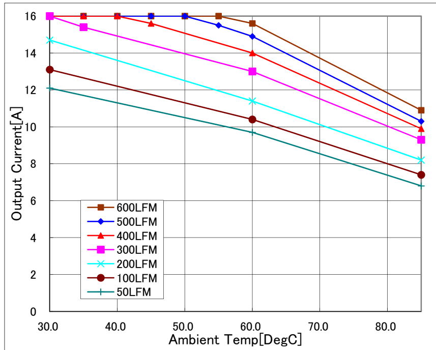
Fig-1: Available load current vs. ambient temperature and airflow rates for Vin=48V. Maximum component temperature \leq 125^{\circ}\text{C}
