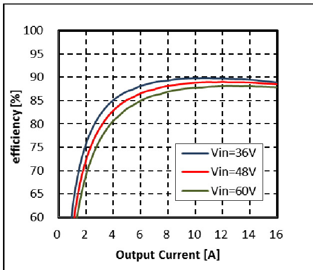
Fig-2: Efficiency vs. load current and input voltage for converter mounted horizontally with airflow from pin 1 to pin 3 at a rate of 400LFM (2.0m/s) and Ta=25°C.
