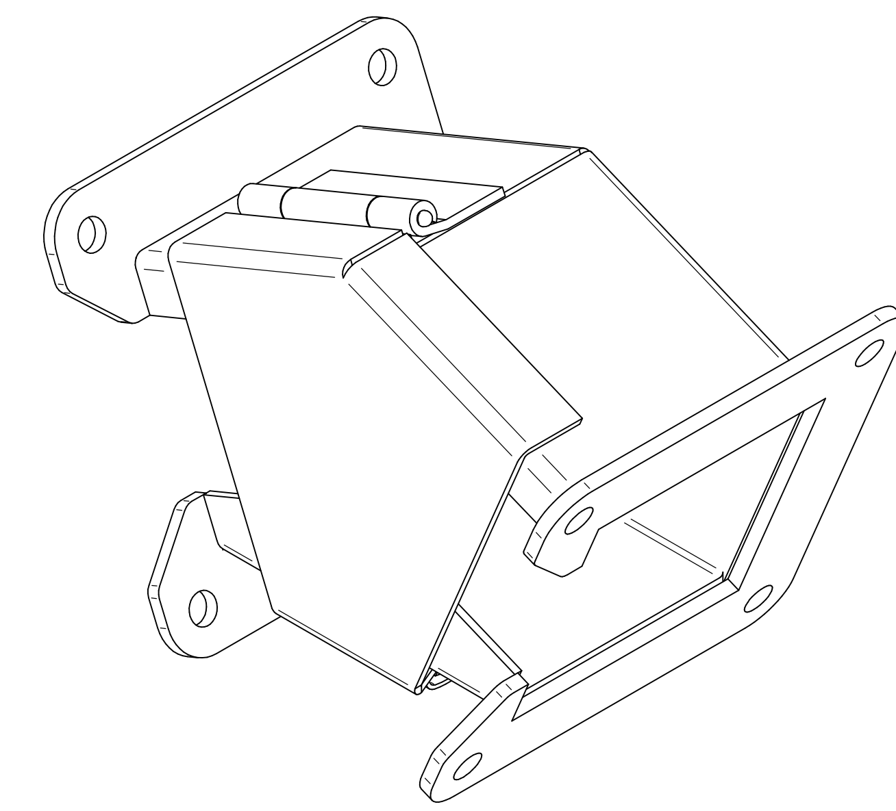
ISOMETRIC VIEWS
