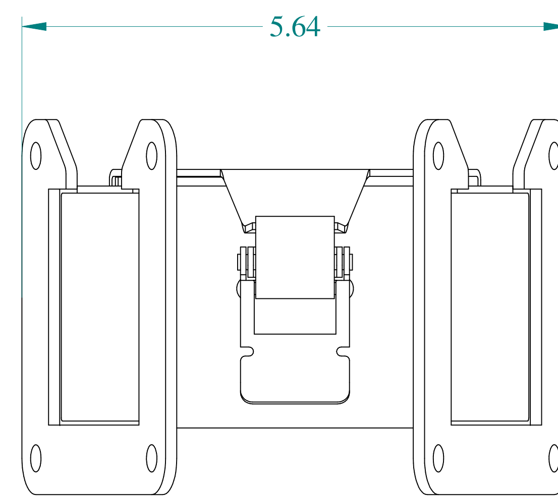
BOTTOM VIEW
