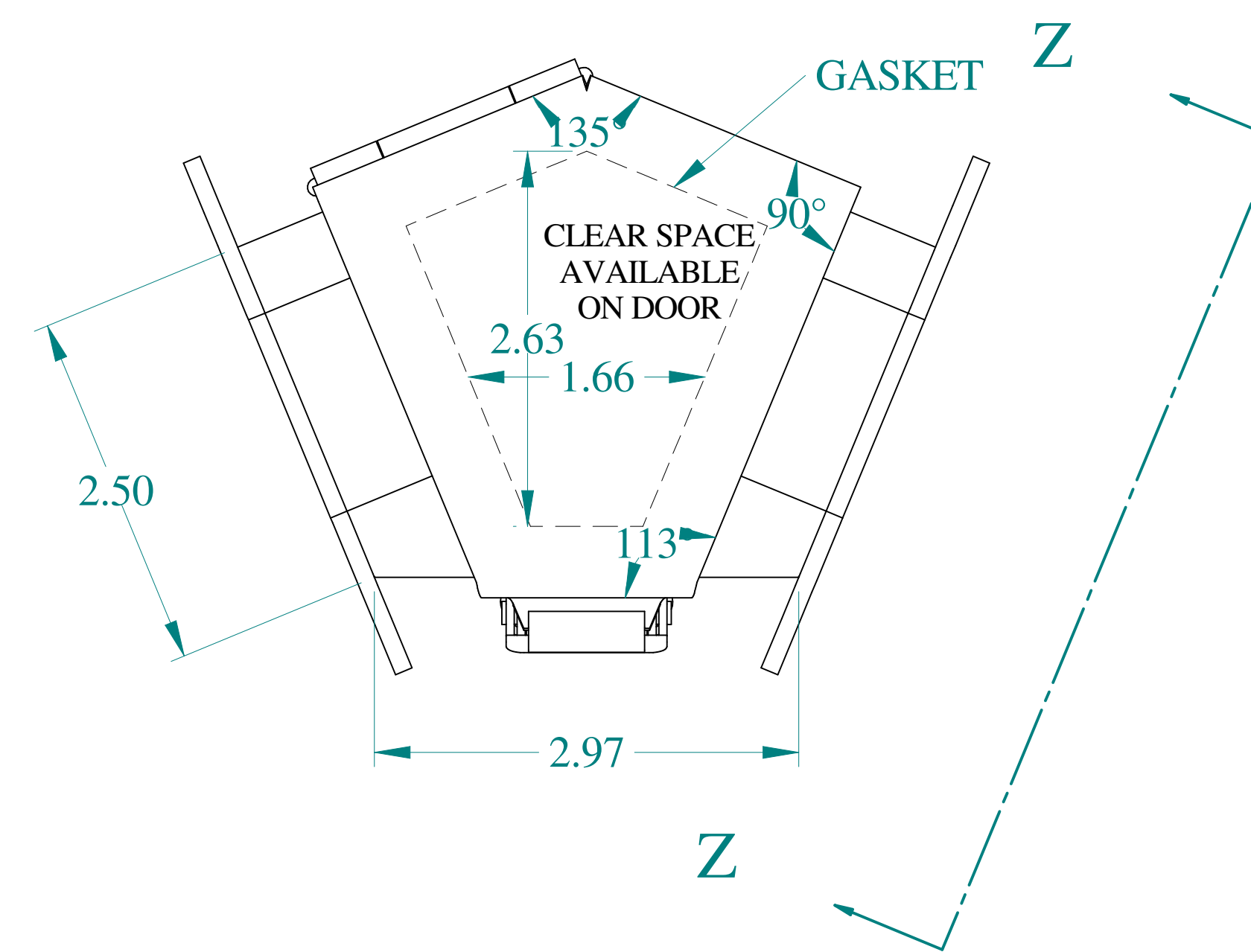
FRONT VIEW
