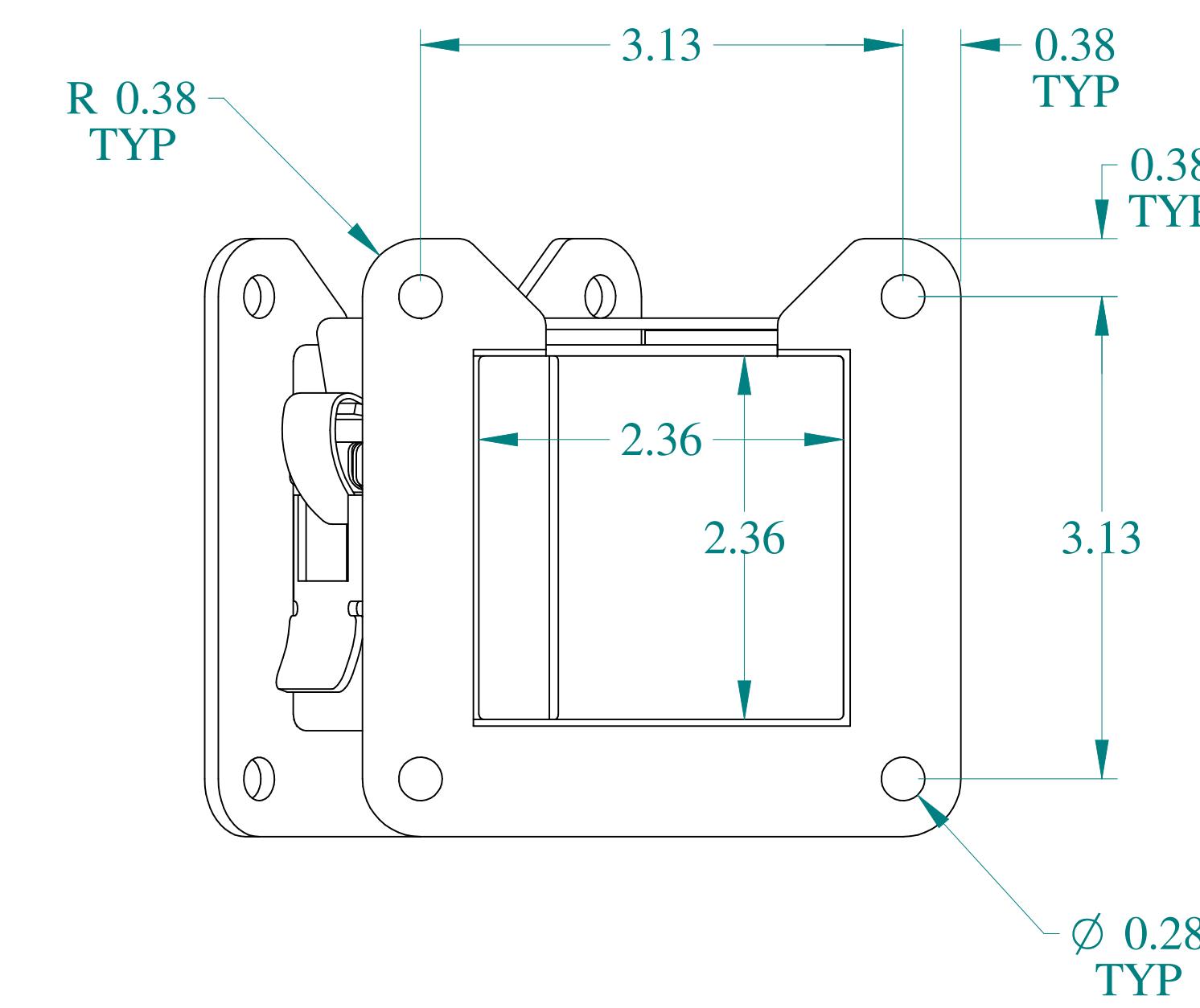
VIEW Z-Z
