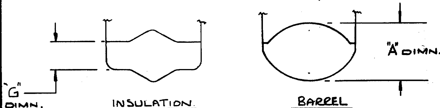
ENLARGED VIEW OF CRIMPS SCALE 10:1
