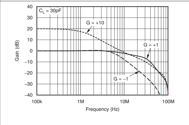
Figure 6-16. Closed-Loop Gain vs Frequency
