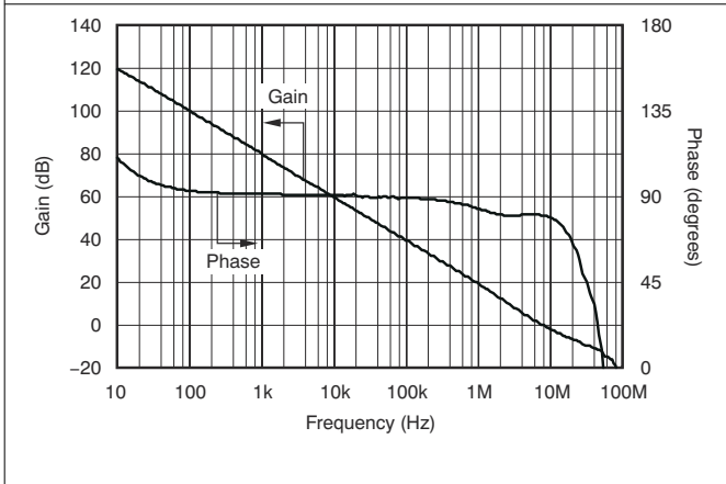
Figure 6-15. Gain and Phase vs Frequency
