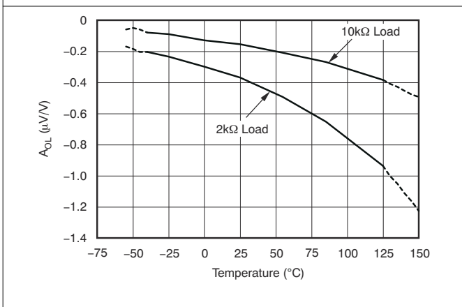
Figure 6-17. Open-Loop Gain vs Temperature
