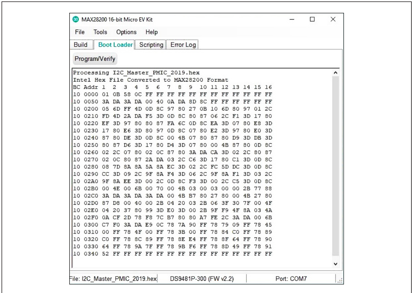
Figure 24. Programming the Device with the Data Pattern
