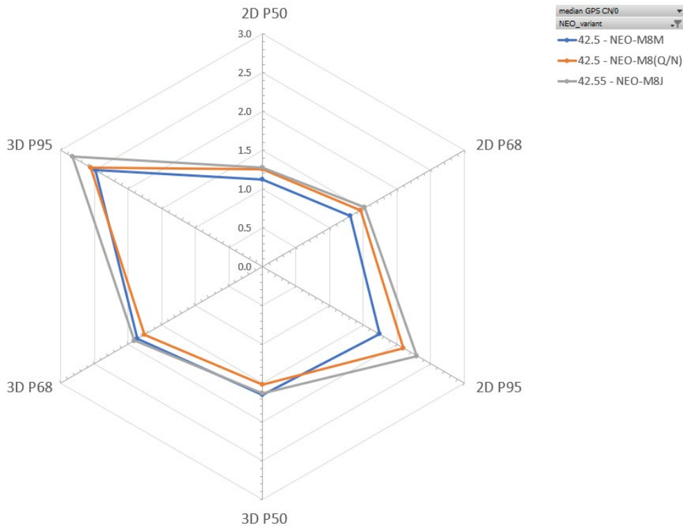
Figure 16: Position error in meters for NEO-M8Q/N, NEO-M8J, and NEO-M8M in percentiles in a highway scenario
