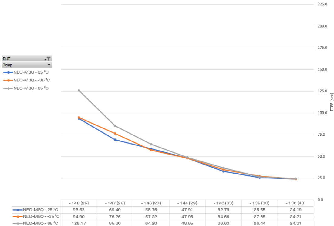
Figure 5: TTFF vs. signal power in dBm and equivalent C/N0 inside parentheses for NEO-M8Q/N during cold starts at +25, -35, and +85 °C
