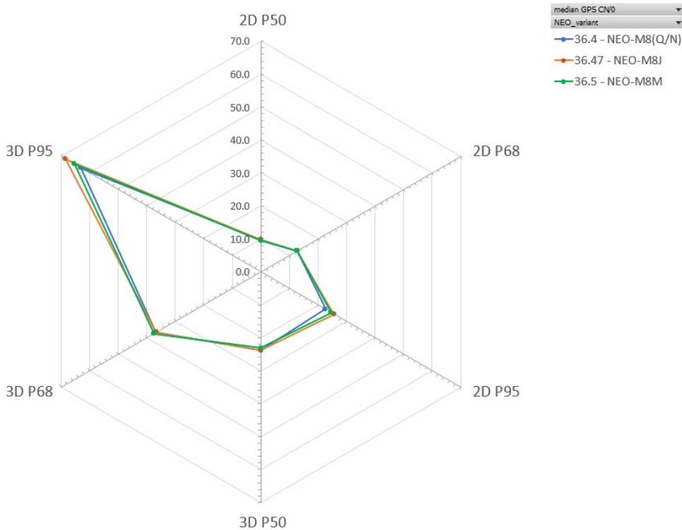
Figure 11: Position error in meters for NEO-M8Q/N and NEO-M8M in percentiles. Urban canyon scenario.
