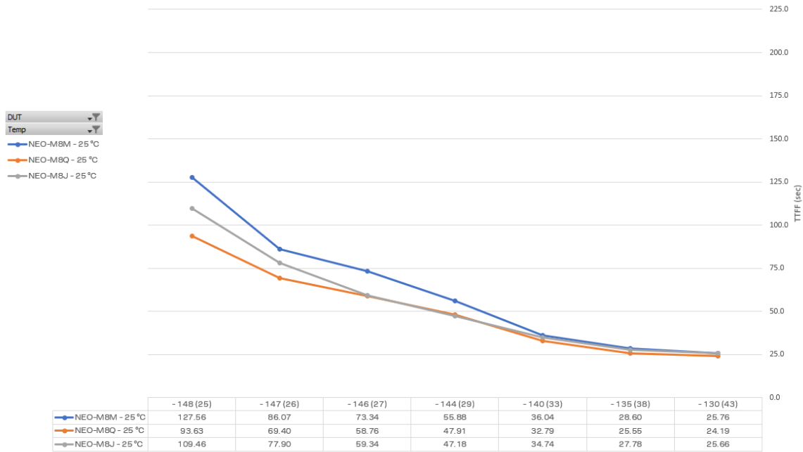
Figure 2: TTF vs. signal power in dBm and equivalent C/N0 inside parenthesis for NEO-M8Q, NEO-M8M and NEO-M8J during cold starts 11 (default mode: GPS & GLONASS including QZSS, SBAS)
