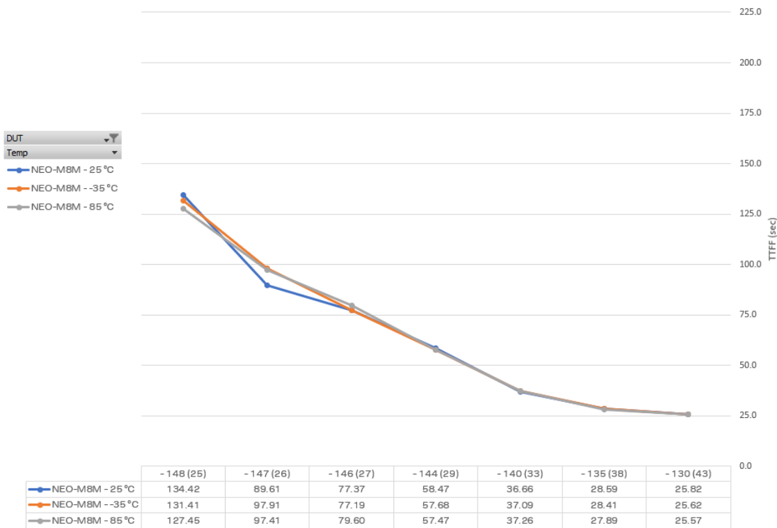
Figure 4: TTFF vs. signal power in dBm and equivalent C/N0 inside parentheses for NEO-M8M during cold starts at +25, -35, and +85 °C
