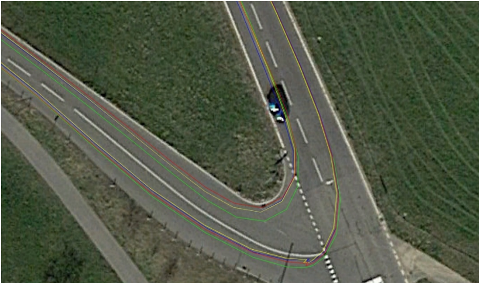
Figure 8: NEO-M8(Q/N), NEO-M8M, NEO-M8J, and reference position tracks in curves. Same color pattern as in Figure 7.
