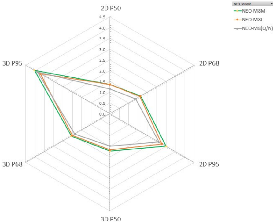
Figure 6: Position error in meters for NEO-M8Q/N and NEO-M8M in percentiles. Rural areas with good signal reception conditions.
