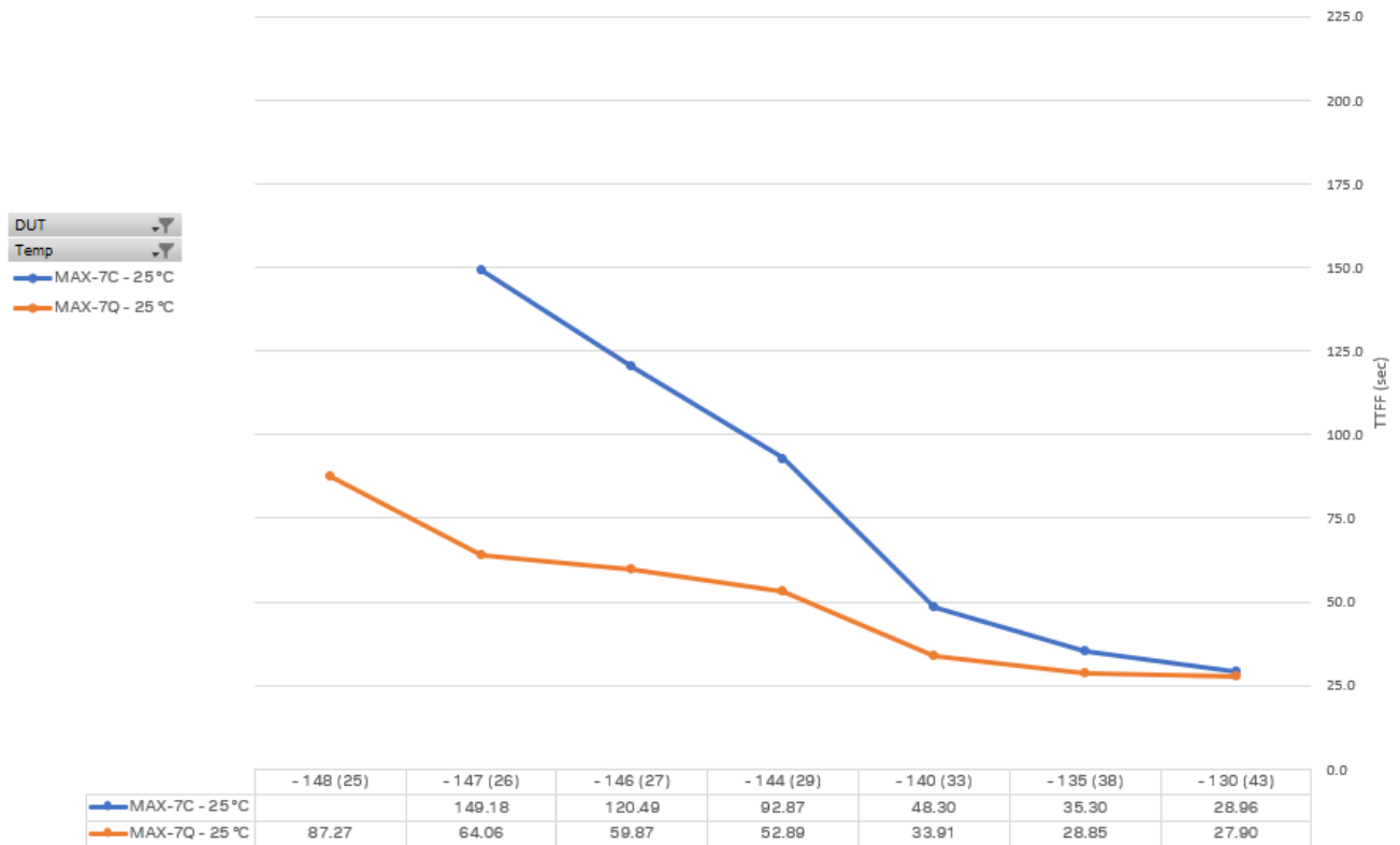
Figure 17: TTFF vs. signal power in dBm and its equivalent in C/N0 inside parentheses for MAX-7Q and MAX-7C during cold starts (default mode: GPS & GLONASS including QZSS, SBAS)
