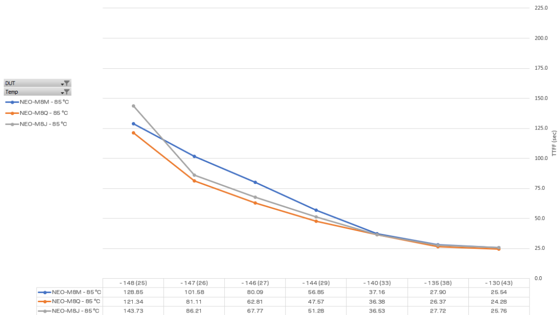
Figure 3: TTF vs. signal power in dBm and equivalent C/N0 inside parenthesis for NEO-M8Q, NEO-M8M and NEO-M8J during cold starts 11 (default mode: GPS & GLONASS including QZSS, SBAS) at 85°C
