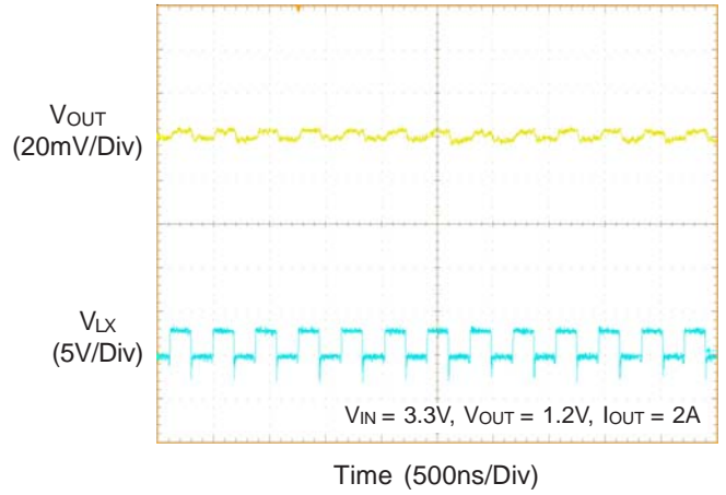
Voltage Ripple
